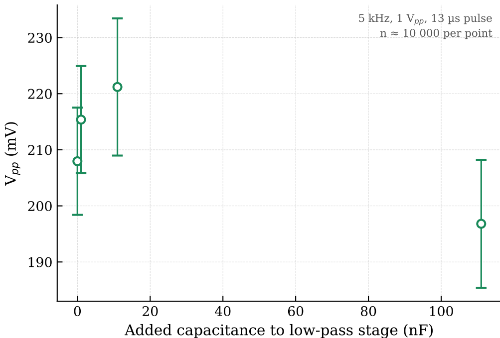
Peak-to-peak voltage vs. low-pass added capacitance
